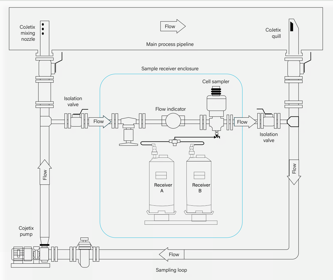
Typical systems schematic (Note: Not to scale).
